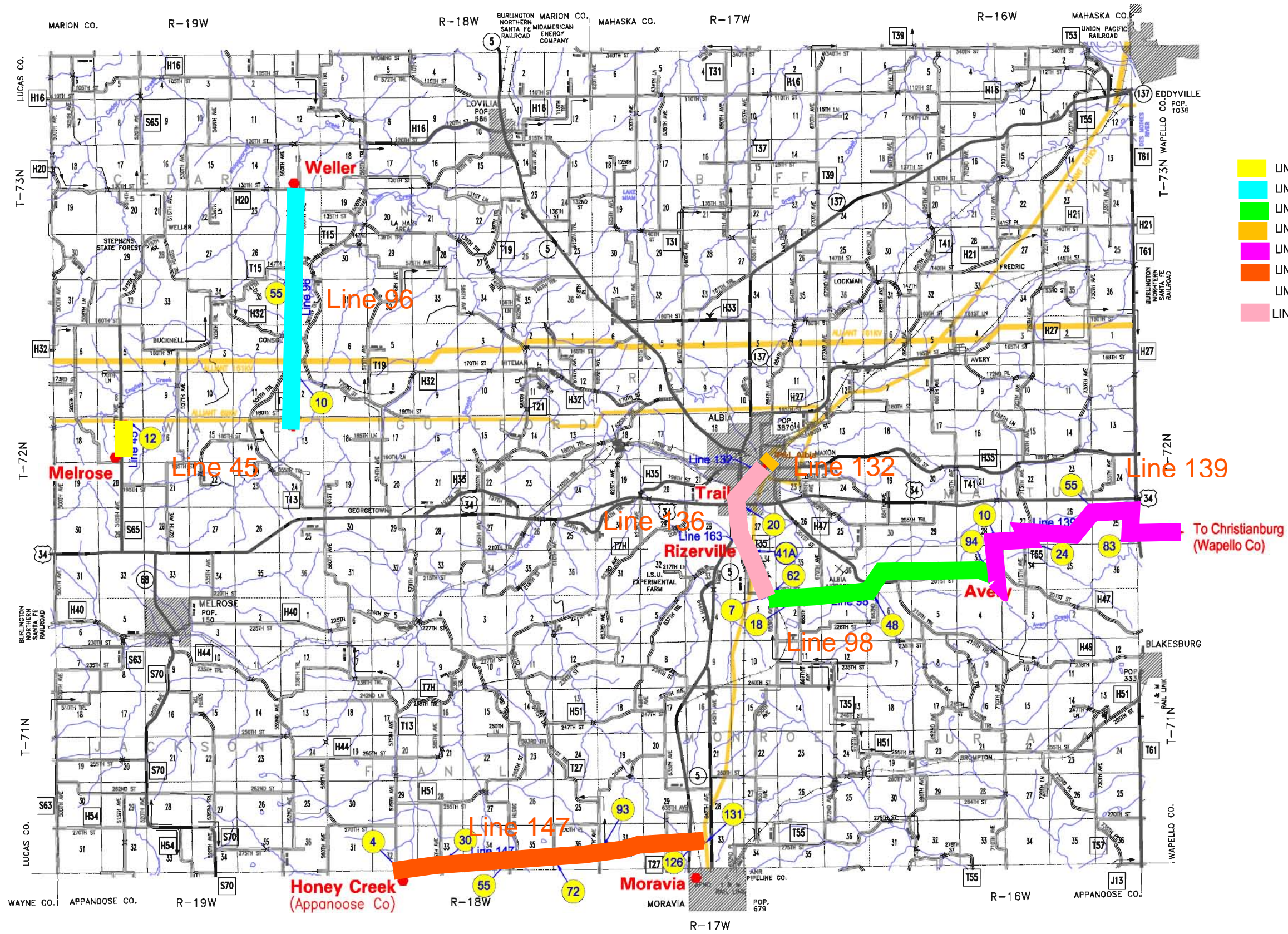
69KV TRANSMISSION LINES IN MONROE COUNTY
