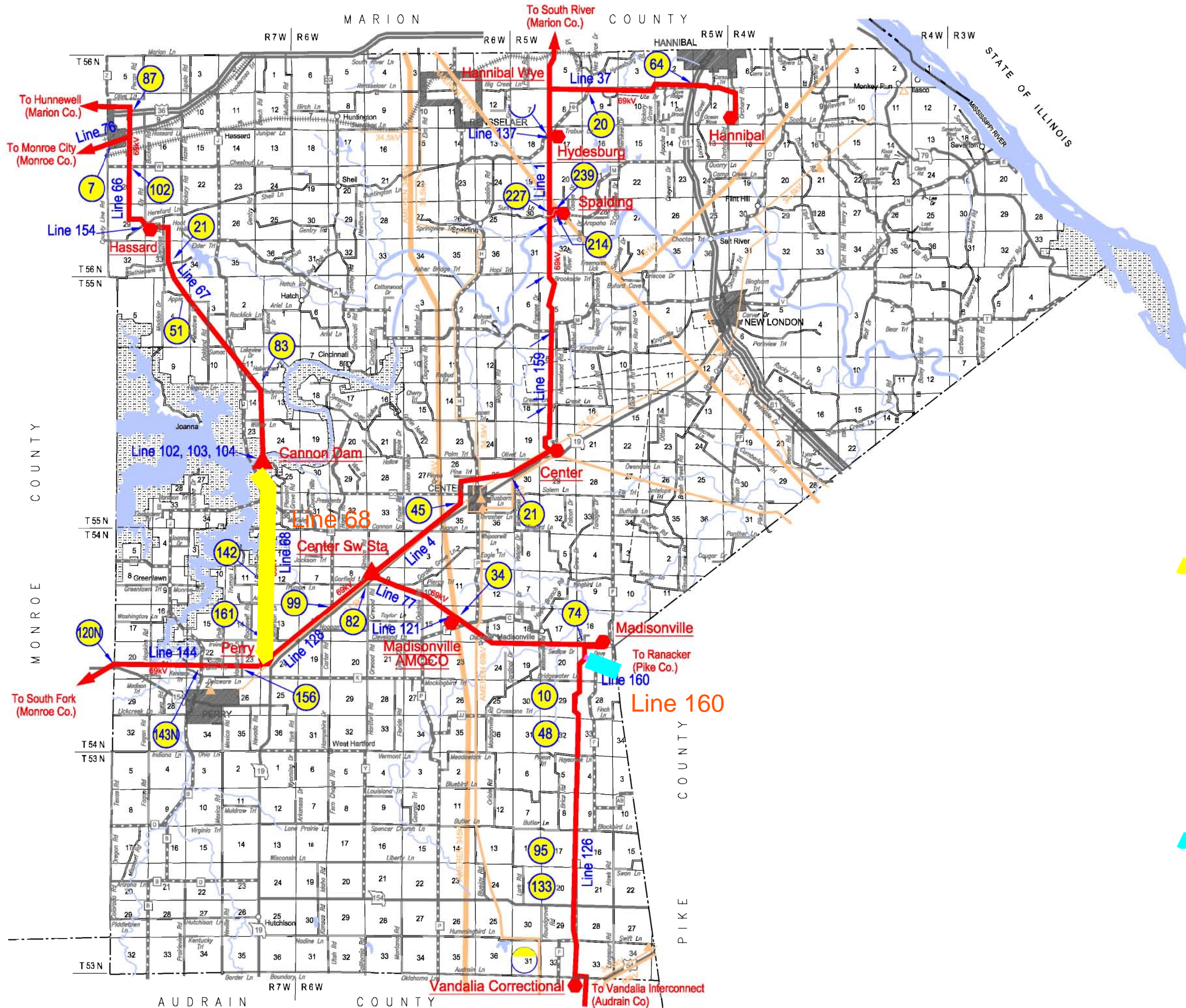
69KV TRANSMISSION LINES IN RALLS COUNTY
